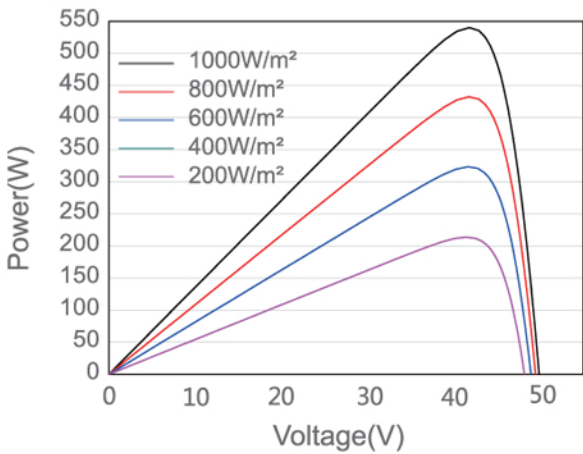
Power-Voltage Curve JAM72S30-540/MR
