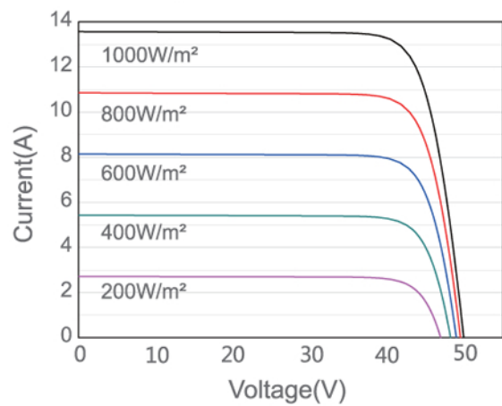
Current-Voltage Curve JAM72S30-540/MR
